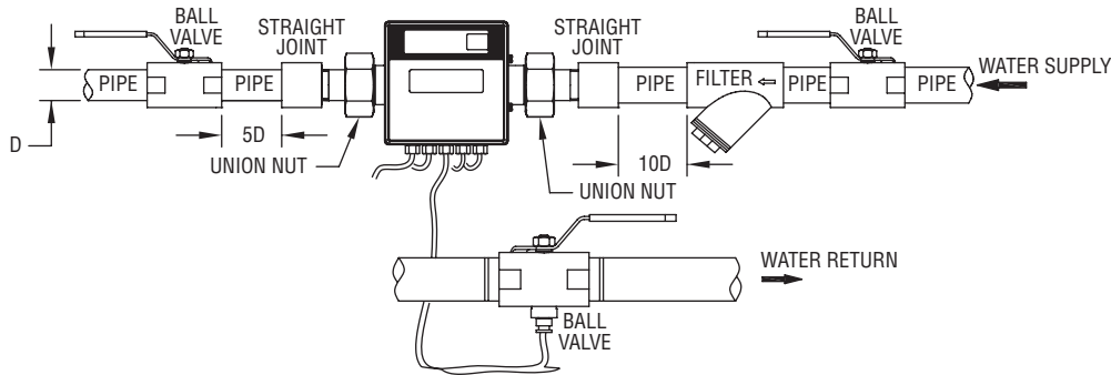
Figure 1: Installation diagram for TUF-150/400
