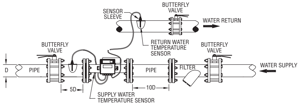
Figure 2: Installation diagram for TUF-500/2000
