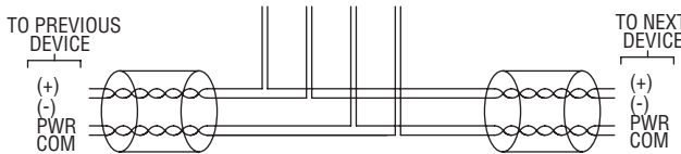
Figure 1: Common local power supply
