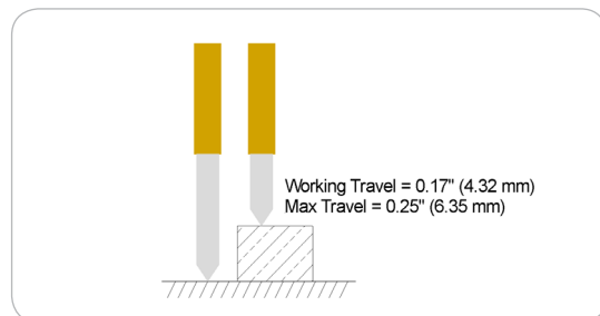
BKP-10 Pin Travel
