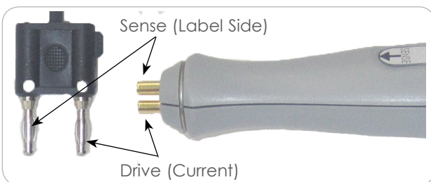
BKP-10 Pinout Information
