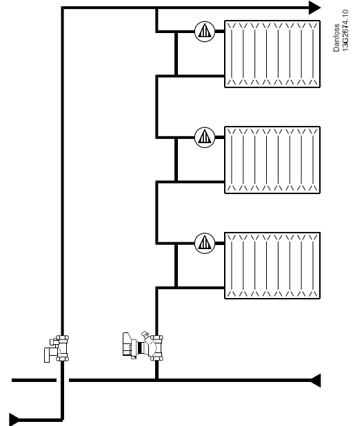
1-pipe system
